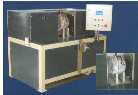
Figure 10-6: Induction die heater (Photo courtesy of IAS GmbH)
